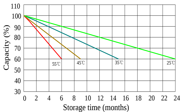
Self-discharge at different temperature
