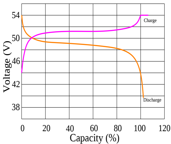
Charge and Discharge at 40°C, 0.5C
